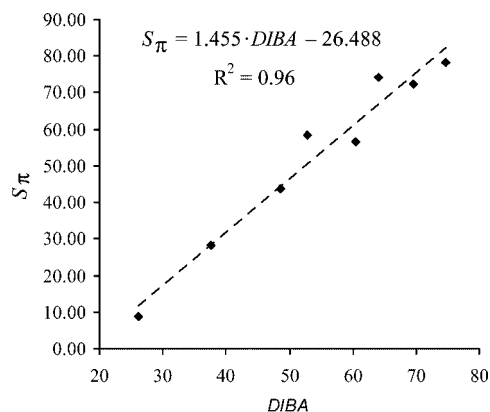
Figure 2. Plot of \pi -strain ( S_\pi ) [kcalmol -1 ] vs. the deviation of the internal bond angle ( DIBA , in degrees) for the complete series of cycloalkynes.
