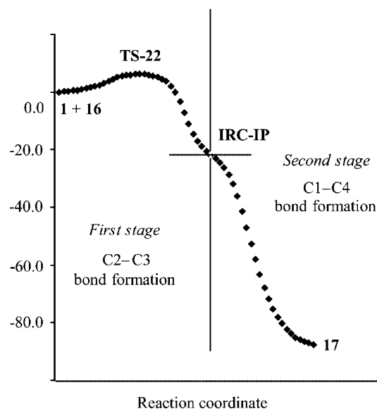
Figure 5. MP2/6-31G* reaction profile for the two-stage, one-step [2+2] cycloaddition between 1 and 16 . IRC-IP corresponds to the inflexion point on the IRC that shares the two-stage regions.
